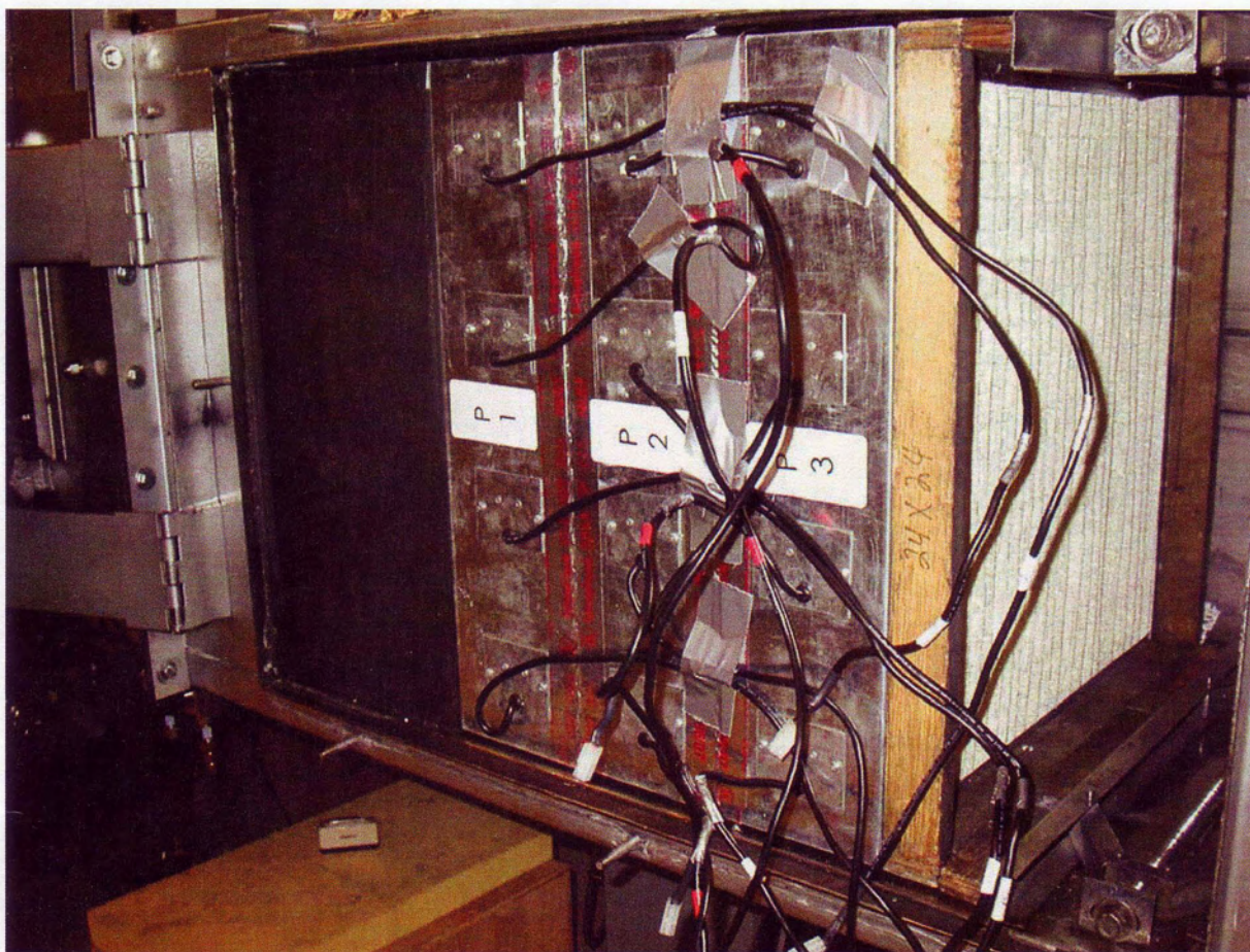
Photograph 4. View of sequential photo-catalytic oxidation sections installed in test duct. Air flow in the test duct is from left to right. The black section directly upstream of the device is the light baffle. Adjustable mechanical clamps and wooden force-transfer elements visible at the right of the photo secure the test assembly against a gasketed flange within the test duct. The entire side of the test duct section shown is covered by a sealed panel, through which the electrical cords pass.
